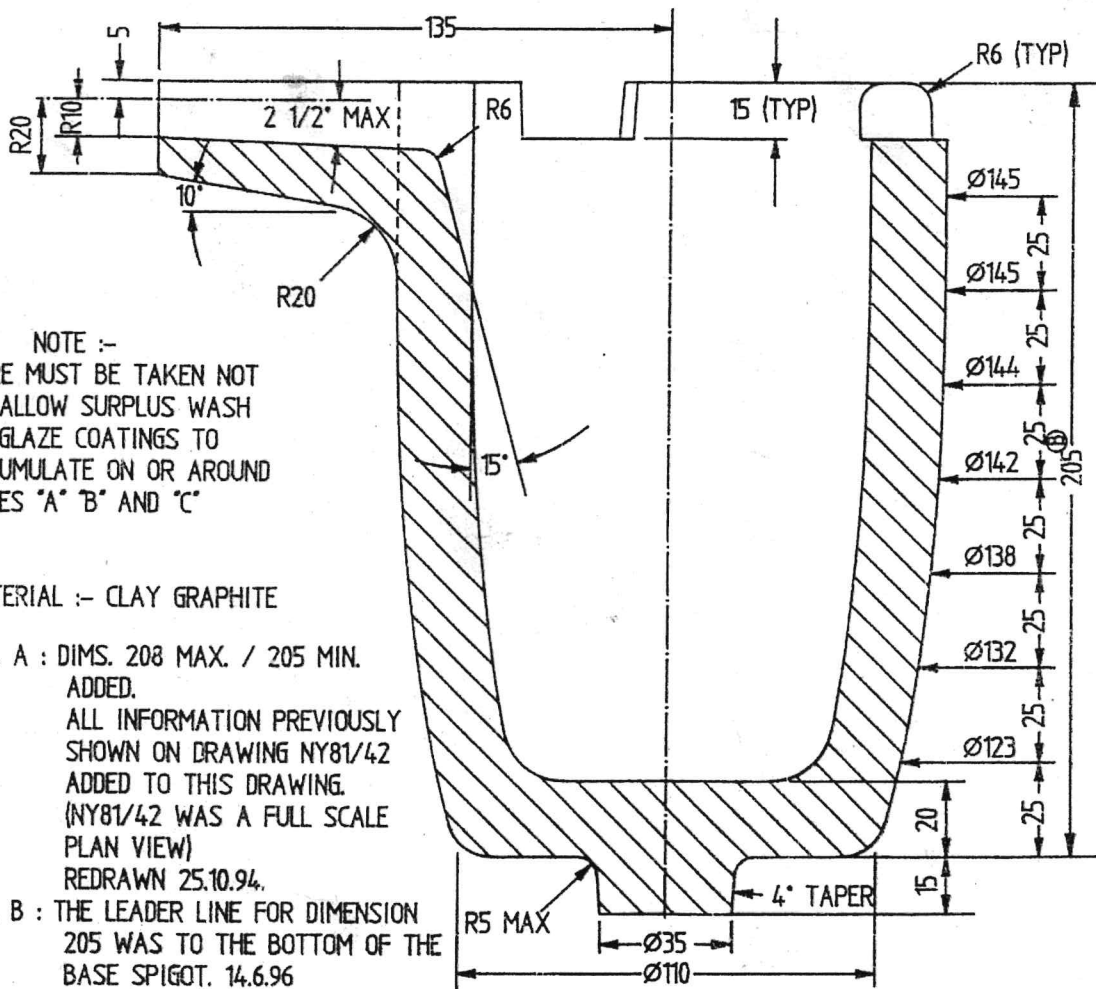
ATP 10 CRUCIBLE (RHODES FLAMEFAST FURNACE)
